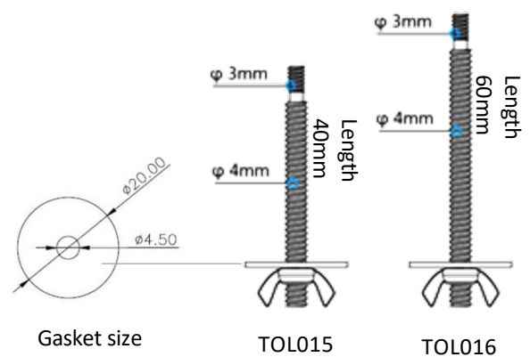
Screw installation options
