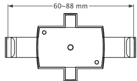
ARK120W-S Horizontal square 2-arm holder
