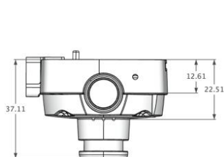
ROX750W
