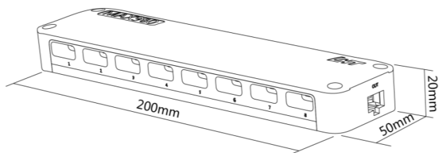
8-puertos FOX980
