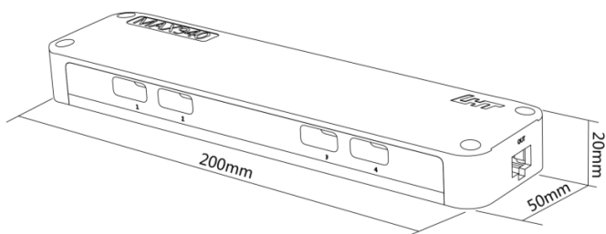
4-puertos FOX940
