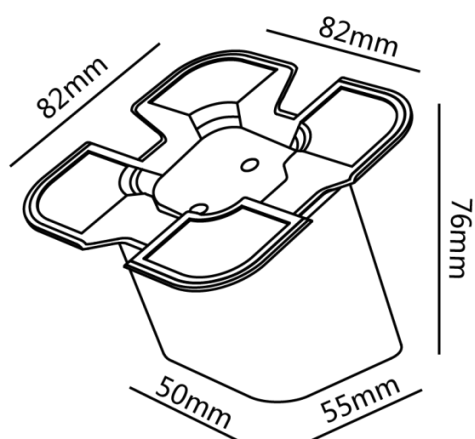
Soporte horizontal 22.5° Tablet FOX715
