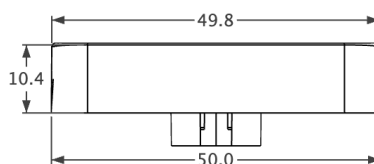
iBox410W Vista frontal
