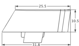
iBox410W Vista lateral
