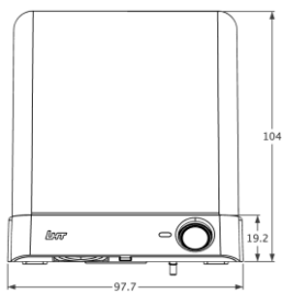
iBox090T Vista frontal
