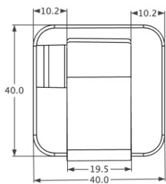
iBox430W vista superior
