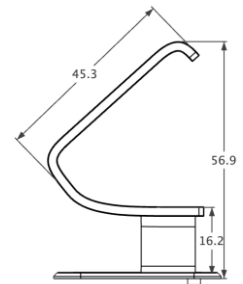
iBox430W Vista lateral
